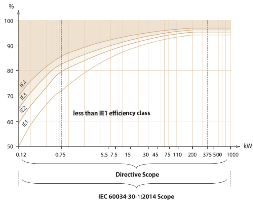
Efficiency levels for 4 pole motors (IEC 60034-30-1:2014)
