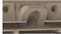
The lifting lugs on the aluminium motors of the frame sizes 132, 160, 180, 200 and 225 are shown in the picture.
